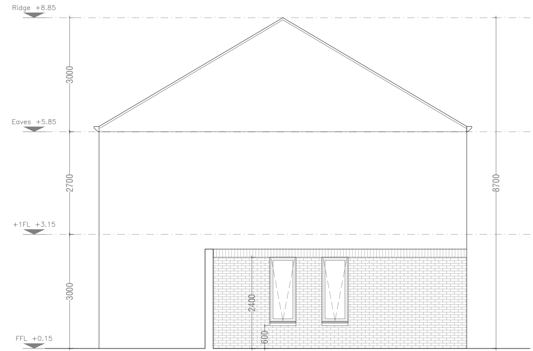
House Type K Semi-Detached Side Elevation
