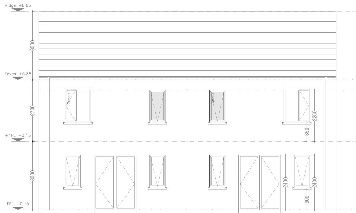
House Type K Semi-Detached Rear Elevation
