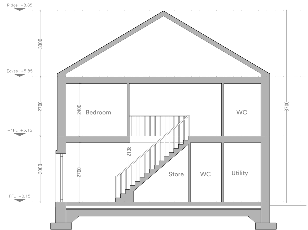
House Type K Semi-Detached Section A.A
